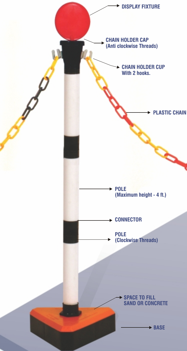
STANDARD STAND POLE ASSEMBLY CONSISTING OF 3 POLES (3' HEIGHT)
